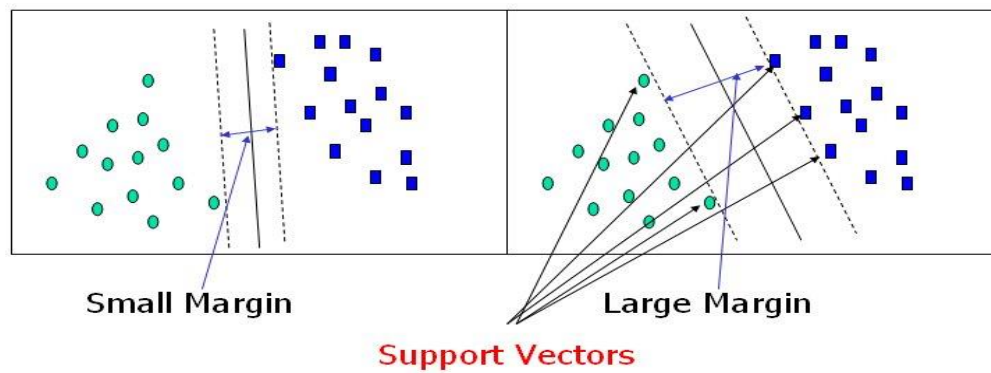
Figure 2. The trade off margin choice
